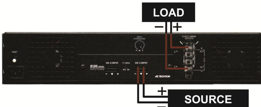
Figure 2.6 – System Wiring
