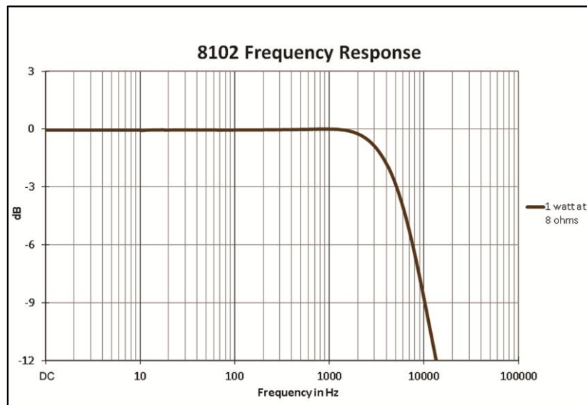
Figure 7.1 – Typical Frequency Response
