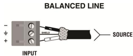
Figure 2.2 - Balanced Input Connector Wiring
