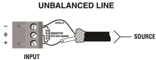
Figure 2.3 - Unbalanced Input Connector Wiring
