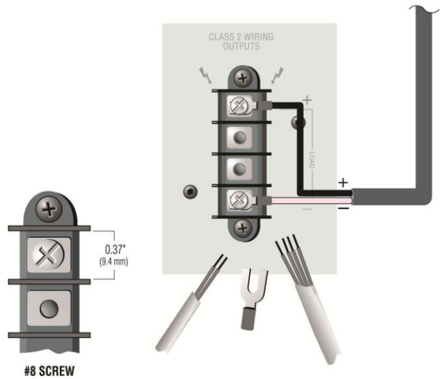
Figure 2.5 – Typical Output Connector Wiring
