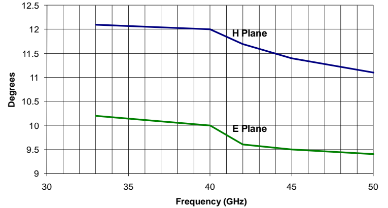
ATH33G50 3dB Beamwidth
