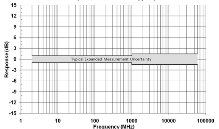
FL7060 Typical Calibrated Frequency Response (with correction factors applied)
