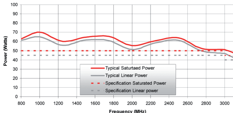
CBA 3G-050 Performance Data
