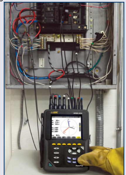
Real-time phasor diagram display.
