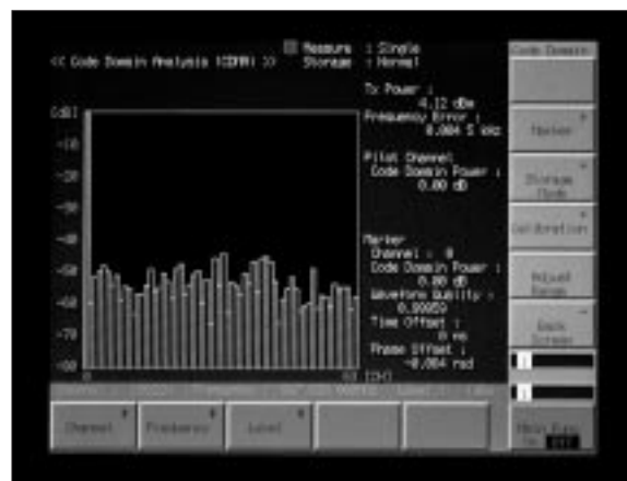
Code domain power measurement
