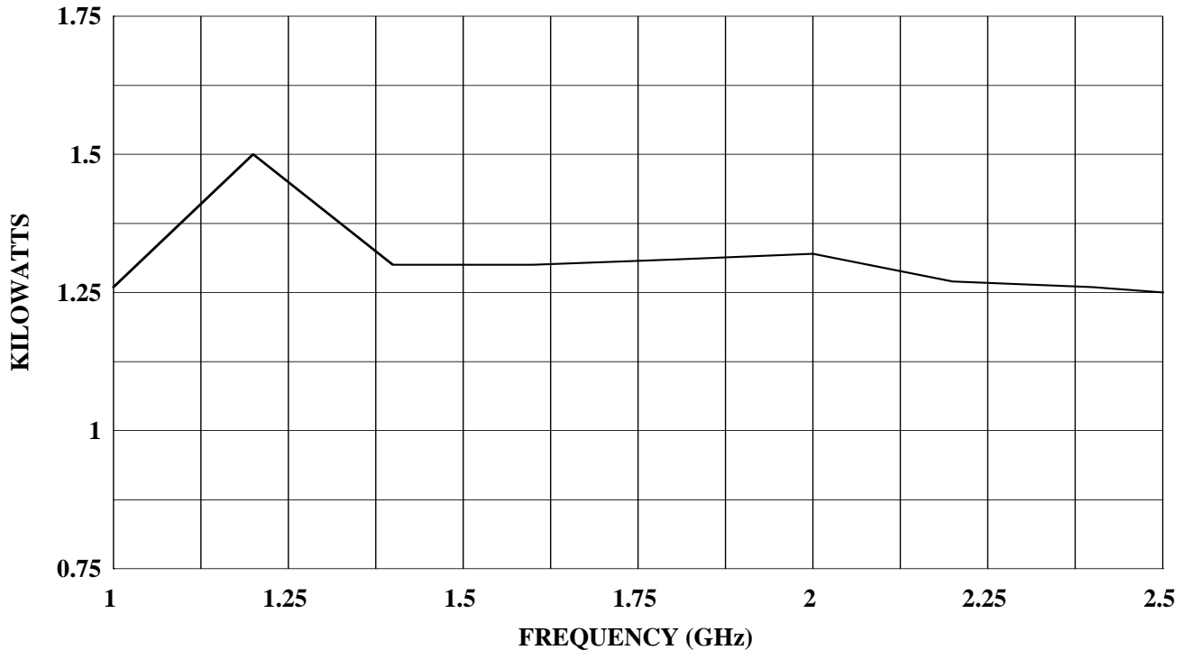
1000TP1G2z5 TYPICAL POWER OUTPUT
