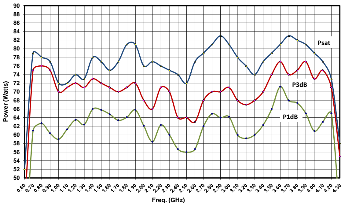
MODEL 60S1G4A TYPICAL POWER OUTPUT
