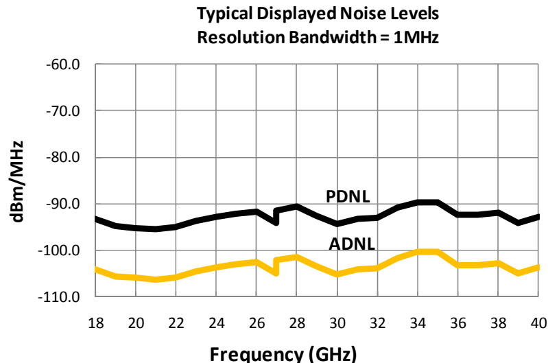
Fig. 2. Typical Displayed Noise Levels when integrated with the DER2018A
