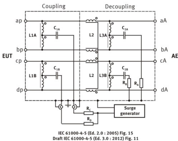
Fig. 11 Draft IEC 61000-4-5 (Ed. 3.0 :2012)
