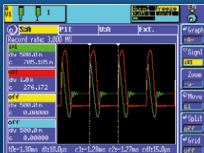
Wave forms of current and voltage
