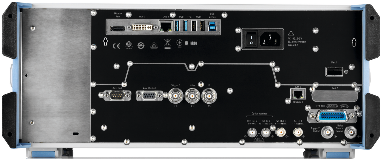
Rear view of the R&S®FSVA3000
